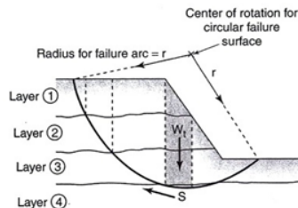
(a) Selection of slices so base arc passes through only one soil type
